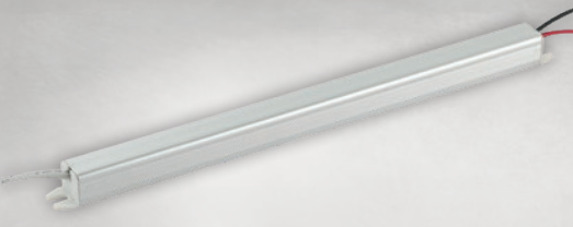
S-72-12V-B LED NAPAJANJE Snaga 72W / 6A Napon 12V Š376*D17*V17mm IP20
