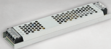
S-150-12V-A LED NAPAJANJE Snaga 150W / 12,5A Napon 12V Š220*D53*V22mm IP20
