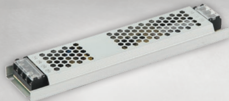
S-200-12V-A LED NAPAJANJE Snaga 200W / 16,7A Napon 12V Š220*D53*V22mm IP20
