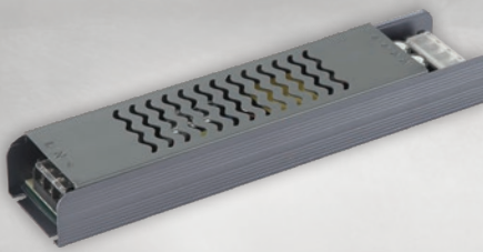
S-200-12V-C LED NAPAJANJE Snaga 200W / 16,7A Napon 12V Š247*D54*V32mm IP20
